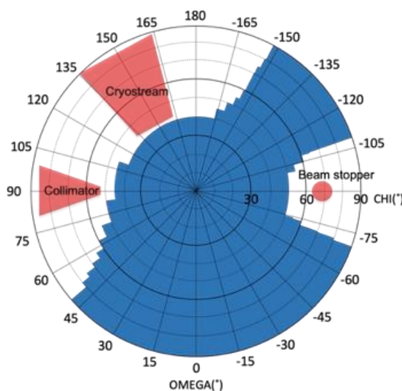
Fig. 5. Range of movement of SMARGON.
