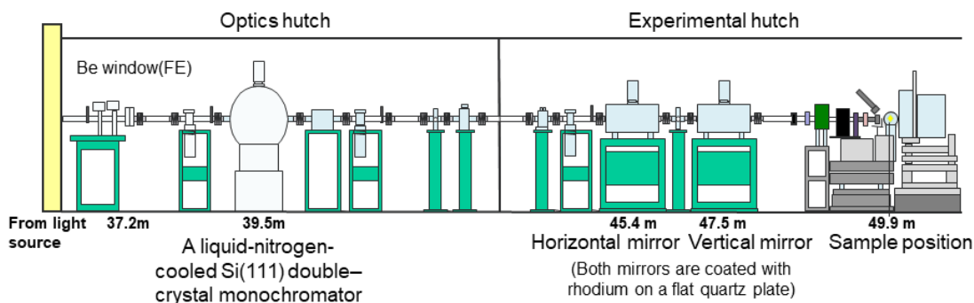
Fig. 1. Beamline components.
