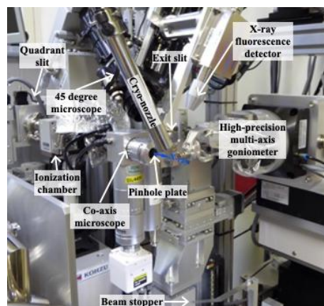
Fig. 3. Goniometer section.
