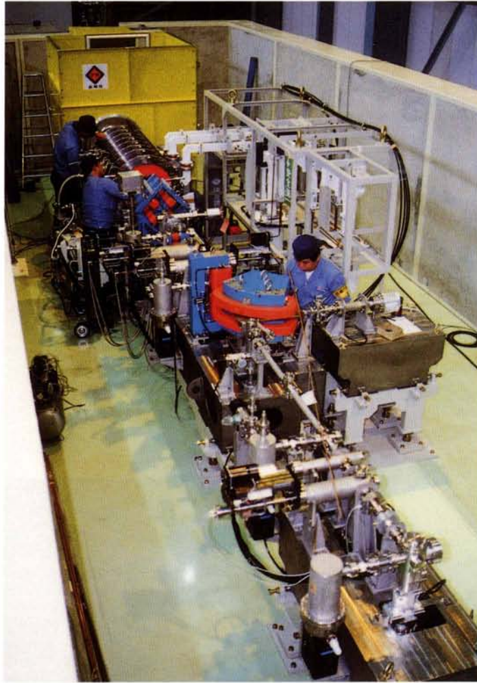
Test operation of the pre-injector of the linac was performed at JAERI, Tokai.
