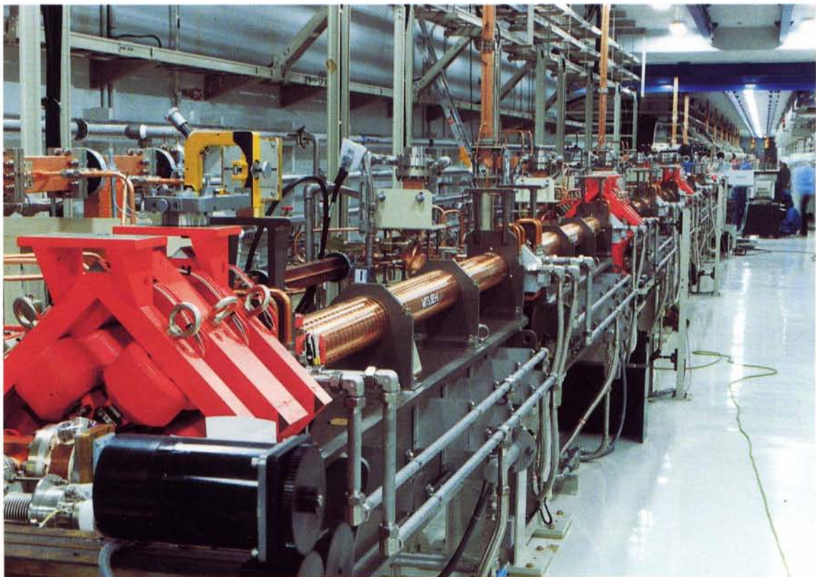
Acceleration sections, quadrupole magnets and waveguides were installed in the linac tunnel below the klystron gallery.
