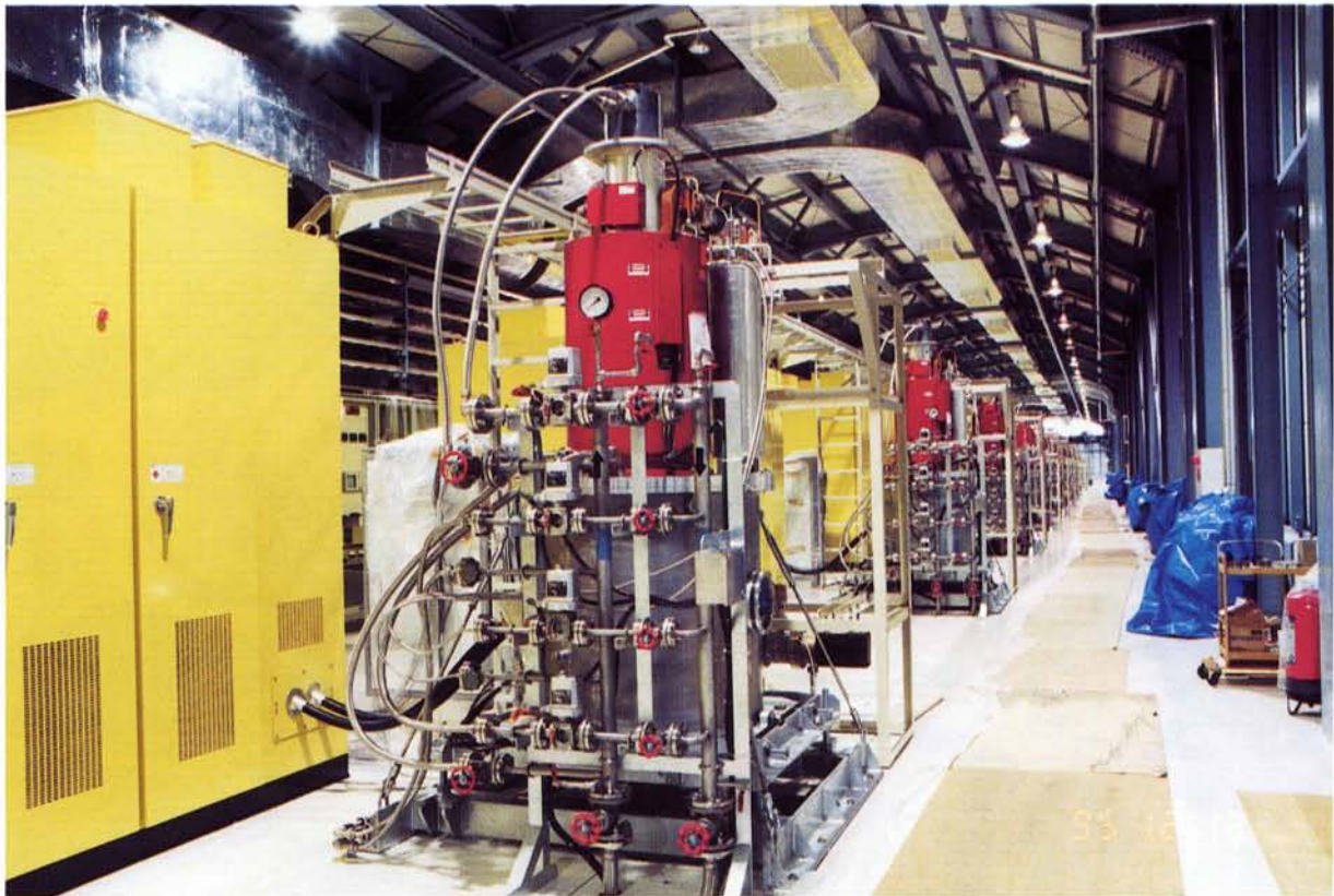
Klystrons and their power supplies of the linac were installed in the klystron gallery.
