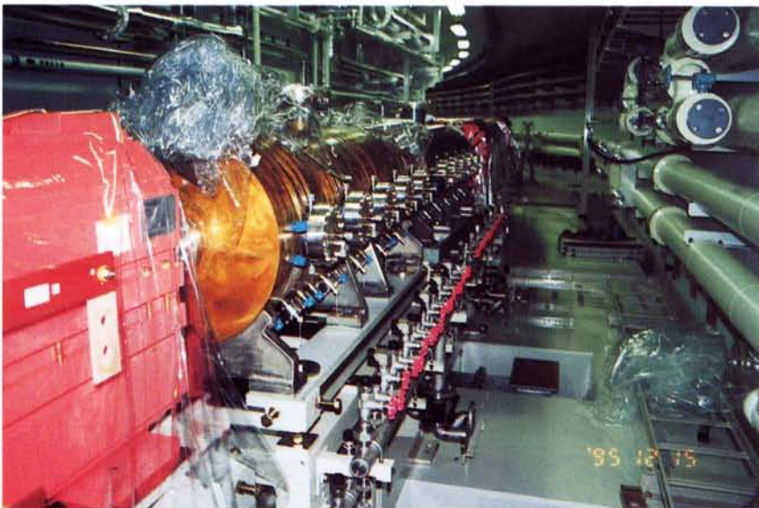
Five-cell cavities for the synchrotron were fabricated and their performance were tested.
