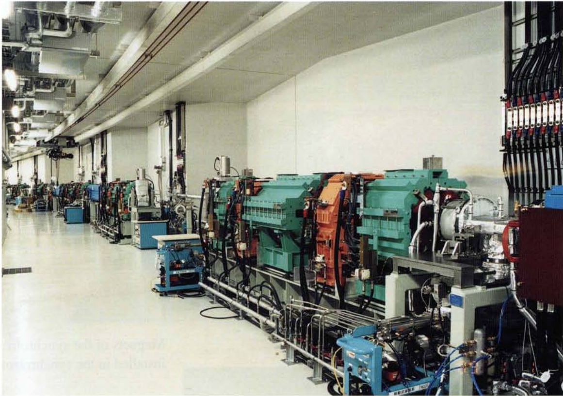
Magnet and vacuum systems were installed and aligned in the storage ring tunnel.
