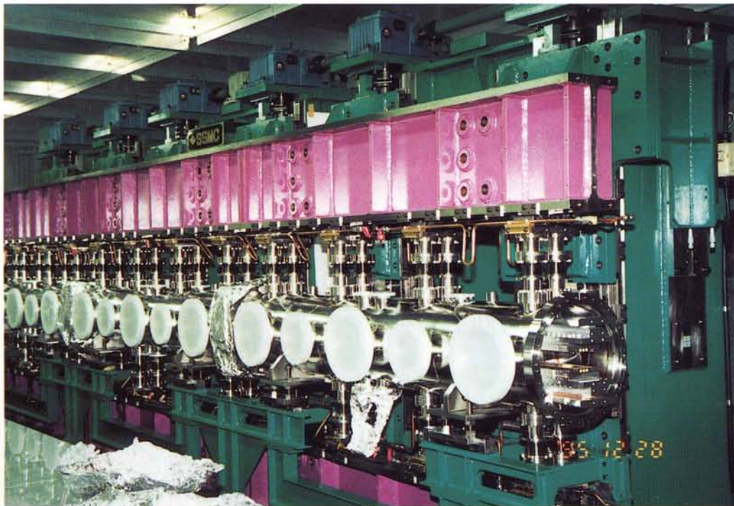
An in-vacuum type insertion device was fabricated, and waiting for field measurement and vacuum test.
