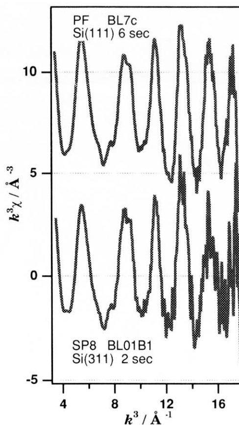
Fig.1 Mo K-edge XAFS spectra of Mo/SiO 2 catalyst. The experimental conditions for both cases. are depicted in the figure.
