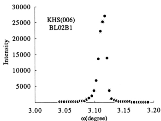
Fig. 1 co-scan profile of observed (006) reflection
