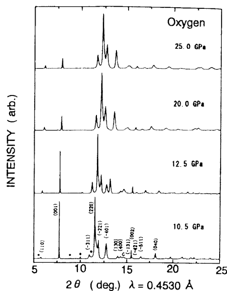
Fig.1. Powder patterns of \epsilon -O 2 phase at various pressure.
