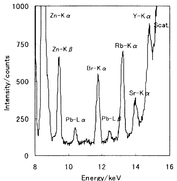
Fig. 2 TXRF spectrum of bovine liver (SRM1577b: sample 360 \mu g)
