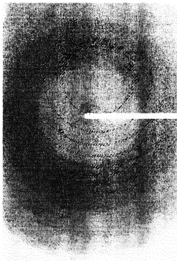
Figure. X-ray diffraction pattern of the reaction center from Chromatium tepidum at the BL41XU beamline.
