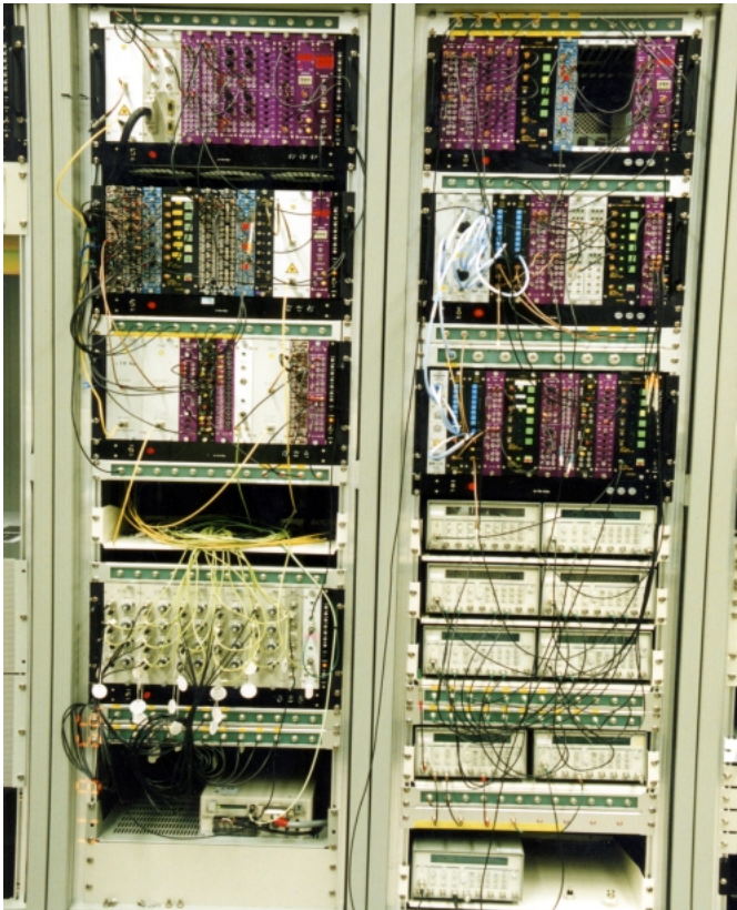
The new timing system of the linac is installed in the beam trigger line of the New SUBARU ring. This timing system is controlled in the central control room.
