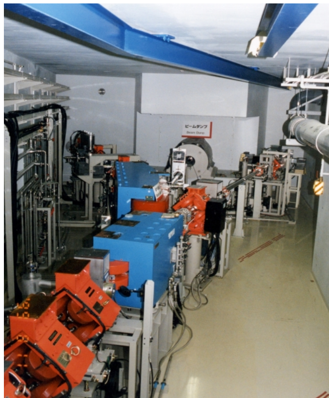
The electron beam from 1GeV linac is divided into synchrotron (LSBT: right side), beam dump (L2: straight), and new beam transport line (L3BT, L4BT: left side) installed in August.
