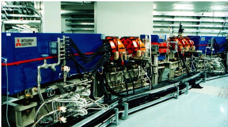
Magnet arrangement of the New SUBARU storage ring.
