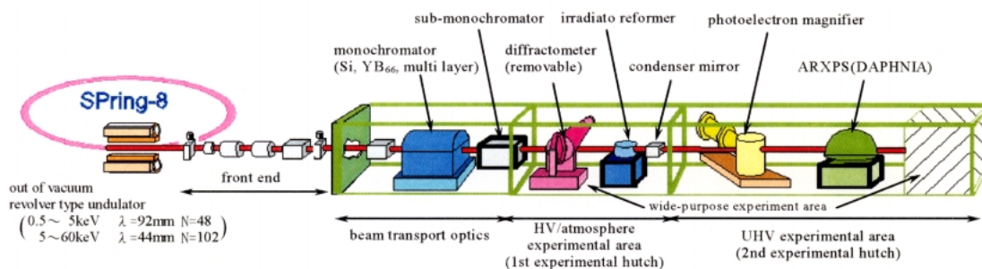
Fig. 1. Outline of WEBRAM.
