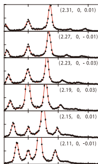
Data from MgB 2 and Supercritical Hg.
