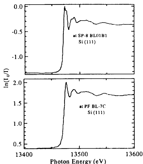
Fig. 1 Br K absorption of KBr at RT.
