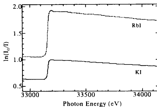
Fig. 2 I K absorption at RT with Si (111).
