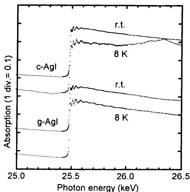
Fig. 1. Ag K-XAFS of crystalline and glassy AgI.
