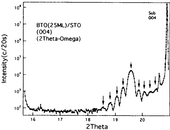
Figure 1 X-ray diffraction profile from 100 \text{\AA} -barium titanate thin film. Peaks from BT are indicated by arrows.
