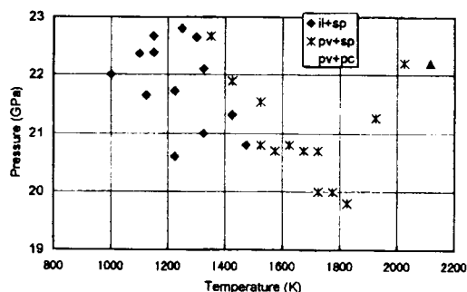
Fig. 2 Observed phases present in the \text{MgSiO}_3 - \text{Mg}_2\text{SiO}_4 system. The diamonds, crosses and triangles denotes phase assemblage of ilmenite+spinel, pervskite+spinel, and perovskite+periclase.
