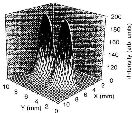
Fig. 1: Intensity distributions of focused 274 keV x-rays. The elliptical multipole wiggler was operated with K_x=0.6 and K_y=11.2 .
