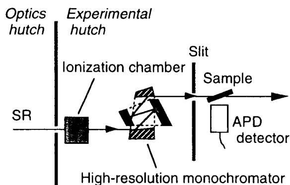
Fig. 1. Experimental setup.
