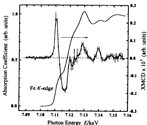
Fig.1. XMCD and XANES at the Fe K -edge in pure Fe.
