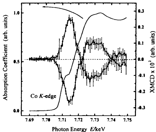
Fig.2. XMCD and XANES at the Co K -edge in pure Co. The reversal of XMCD results from the helicity alternation.
