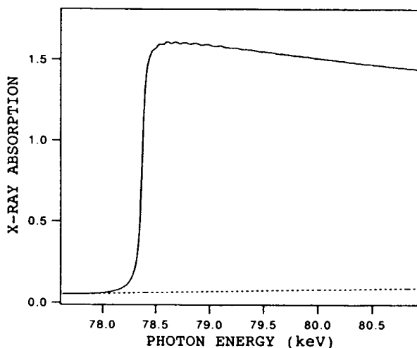
Fig. 1 XAFS spectrum near the Pt-K edge of Pt foil at RT.
