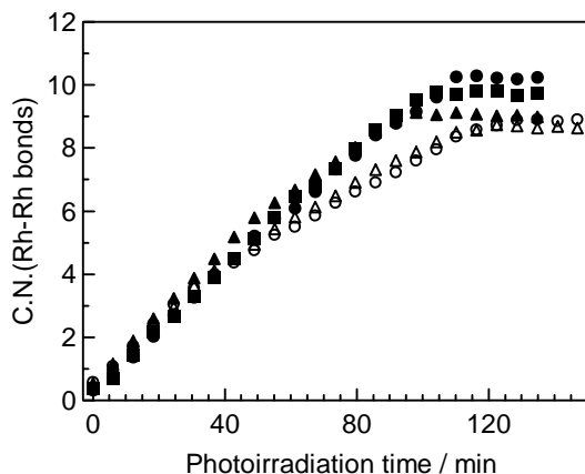
Fig. 6 The variation of the coordination number of Rh-Rh pair with photoirradiation time. Anatase phase: JRC-TIO-8 (●), 1 (▲), 10 (■). Rutile phase: JRC-TIO-3 (○), 6 (△).
