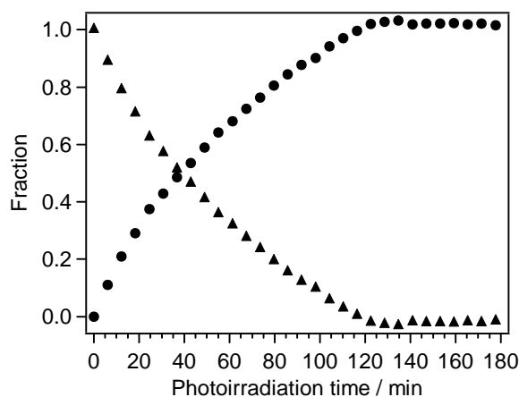
Fig. 3 The variation of the fraction of \text{Rh}^{3+} ion and Rh metal with photoirradiation time. JRC-TIO-3 was used as a photocatalyst.
