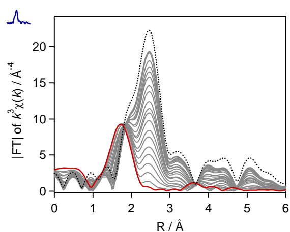
Fig. 5 Series of FT of EXAFS spectra during photodeposition of Rh on JRC-TIO-8, together with Rh foil (dotted line) as a reference. The spectra before photoirradiation (red) and after photoirradiation for 135 min (blue).
