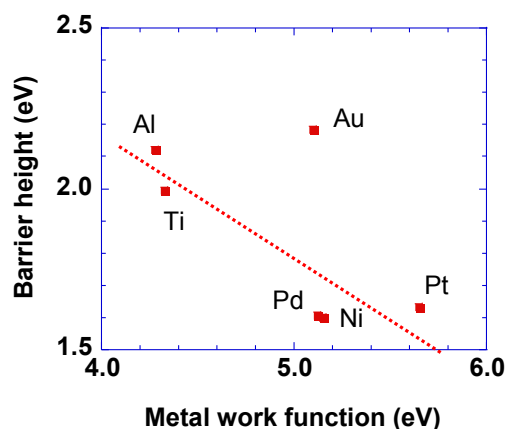
Fig.2 The obtained schottky barrier heights are shown as a function of the work function of the metal.
