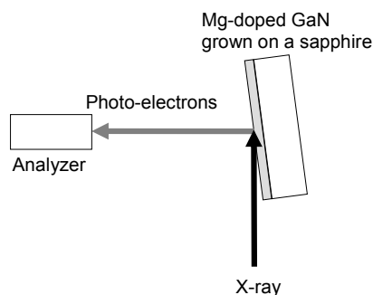
Fig.1 Schematic diagram of sample assembly.
